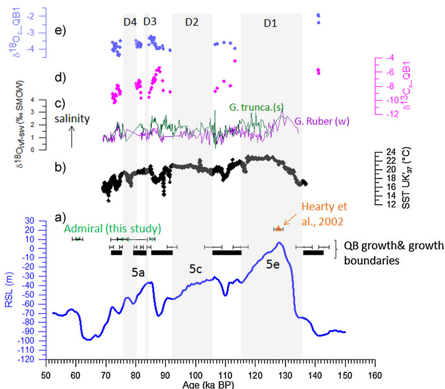
Fig. 6. Comparison of QB growth episodes (discontinuities shown by vertical grey bars) with other data from QB and nearby marine records. a) QB growth periods, with 2 \sigma uncertainty on the boundaries deduced from OxCal model (Fig. 5 and Table S3). The continuous RSL for the Red-Sea (Grant et al., 2012; Siddall et al., 2003) is shown for comparison to allow recognition of highstands identifying the very different isostatic response at this site which is far field and therefore minimally impacted by ice loading/unloading. The comparison is made to the Red Sea sea-level record because it is to date one of the most accepted reference as it is one of the most complete record and because of its independent chronology. Also shown are isolated dates from speleothems at greater altitude on Bermuda than QB; b) UK'37 sea-surface temperature from MD95-2036 (Grant et al., 2013; Lehman et al., 2002); c) \delta^{18}\text{O}_{\text{IVF-SW}} of G. ruber (w) and G. truncatulinoides (s) representing salinity from ODP Site 1058 (Bahr, et al., 2013; Fig. 1 for location); (d) \delta^{13}\text{C} and (e) \delta^{18}\text{O} of the QB speleothem carbonate along a radial transect across B1Cii (this study).
